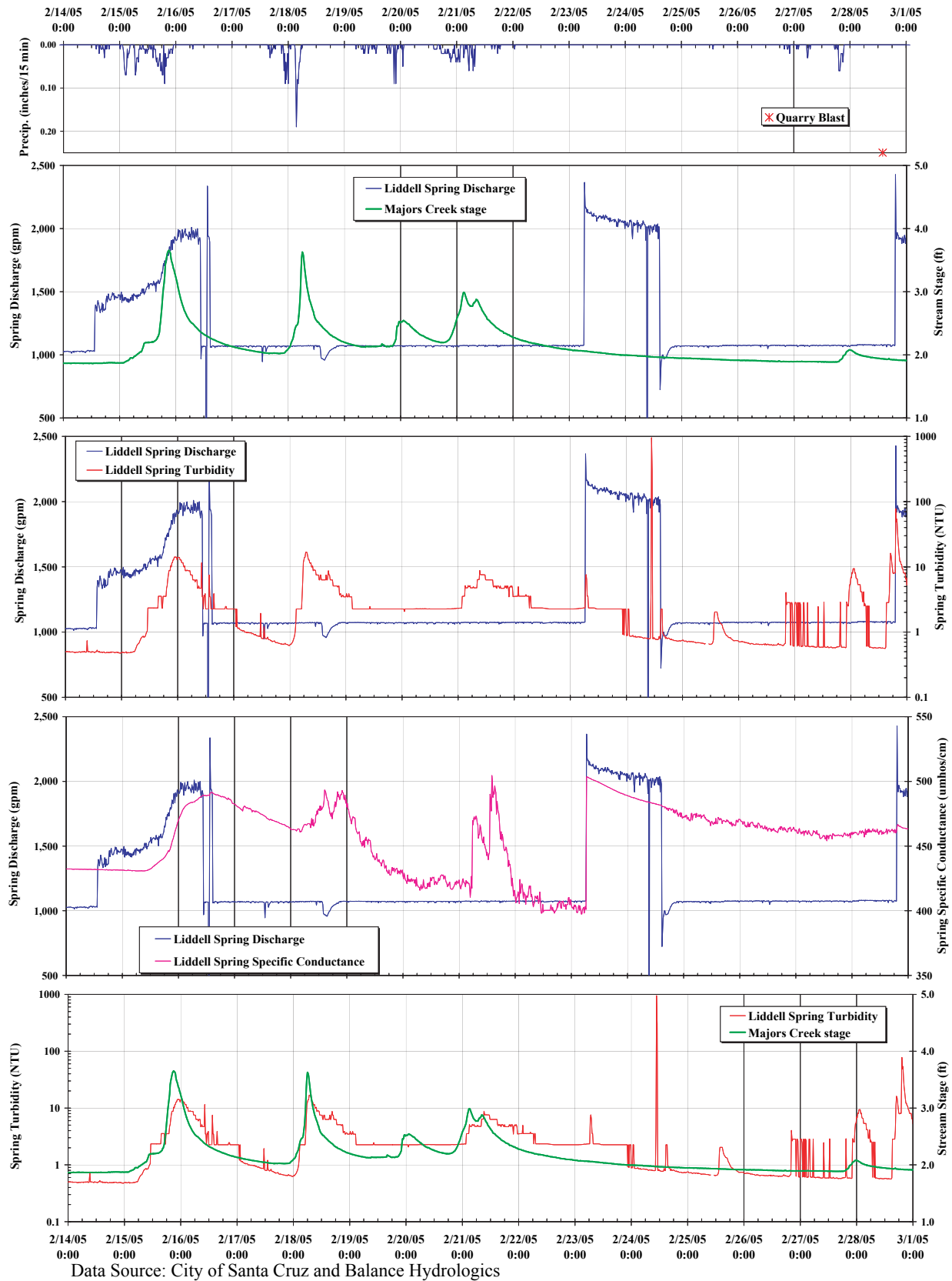
Storm Hydrograph Comparison, February 2005
